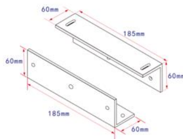
Magnetic lock Z-type bracket (500kg)
