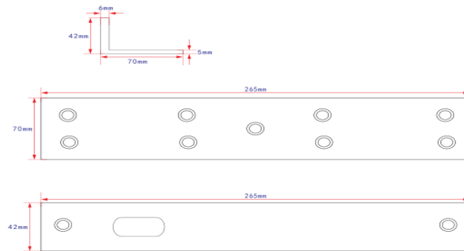
Single-door magnetic lock L-type bracket (500kg)
